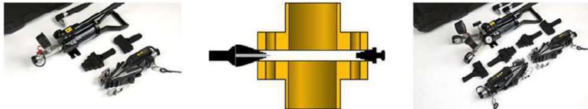
Flange Spreading SWi Wedge Type
